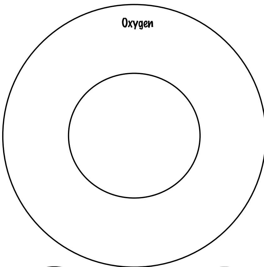
Bohr Model of H 2 O
