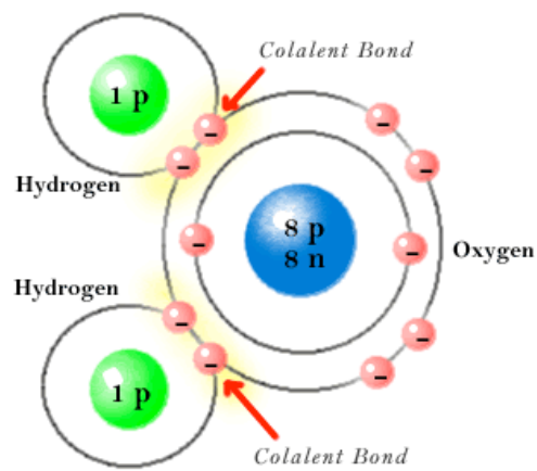
Bohr Model of H 2 O
